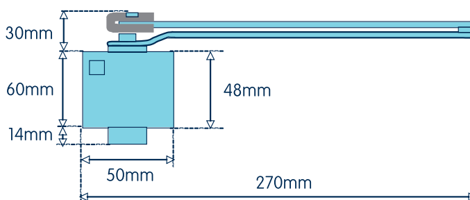
Projecting Arm configuration
